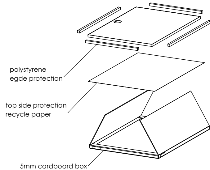
Packing principle
